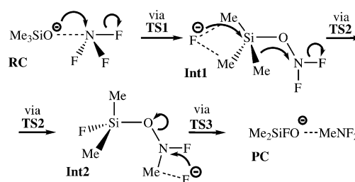
Scheme 1. Proposed reaction mechanism for the Me/F exchange reaction of \text{Me}_3\text{SiO}^- mediated by \text{NF}_3 . Dashed line represents loose bonds between fragments.
