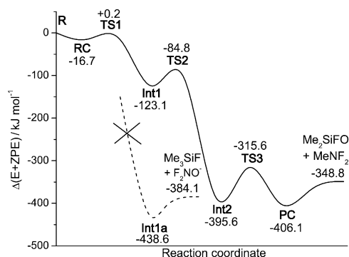
Figure 2. Energy diagram for the \text{Me}_3\text{SiO}^-/\text{NF}_3 reaction calculated at the B3LYP/6-311 + G(3df,2p) level of theory. The dashed line represents the hypothetical (and unobserved) pathway that would lead to the formation of \text{Me}_3\text{SiF} and \text{F}_2\text{NO}^- via adduct Int1a .
